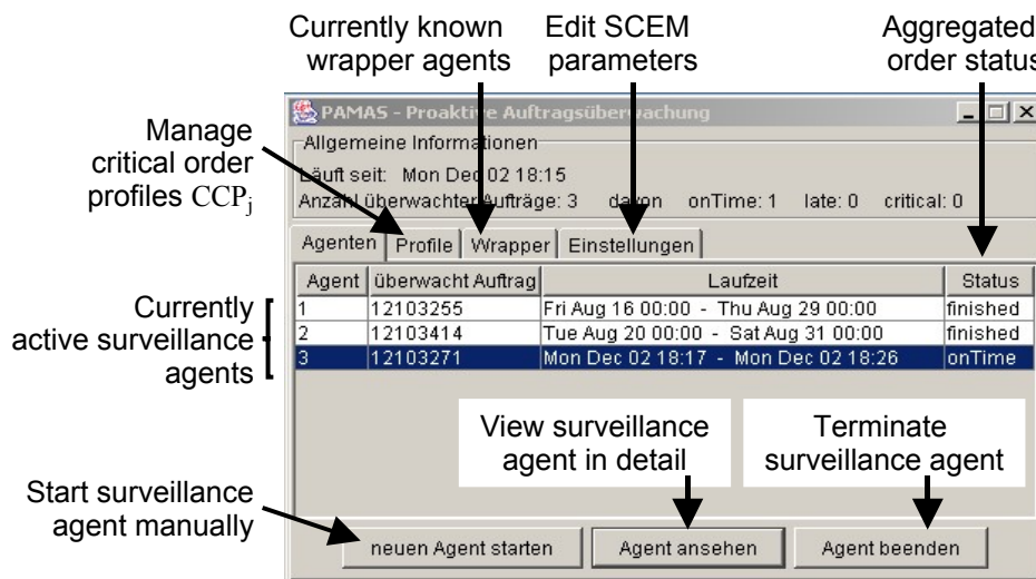
Figure 3: Agent GUI from A4
