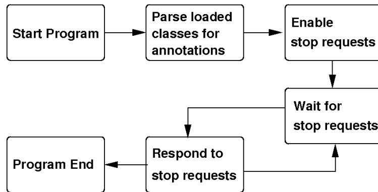
Figure 1: program flow of JPAPA
