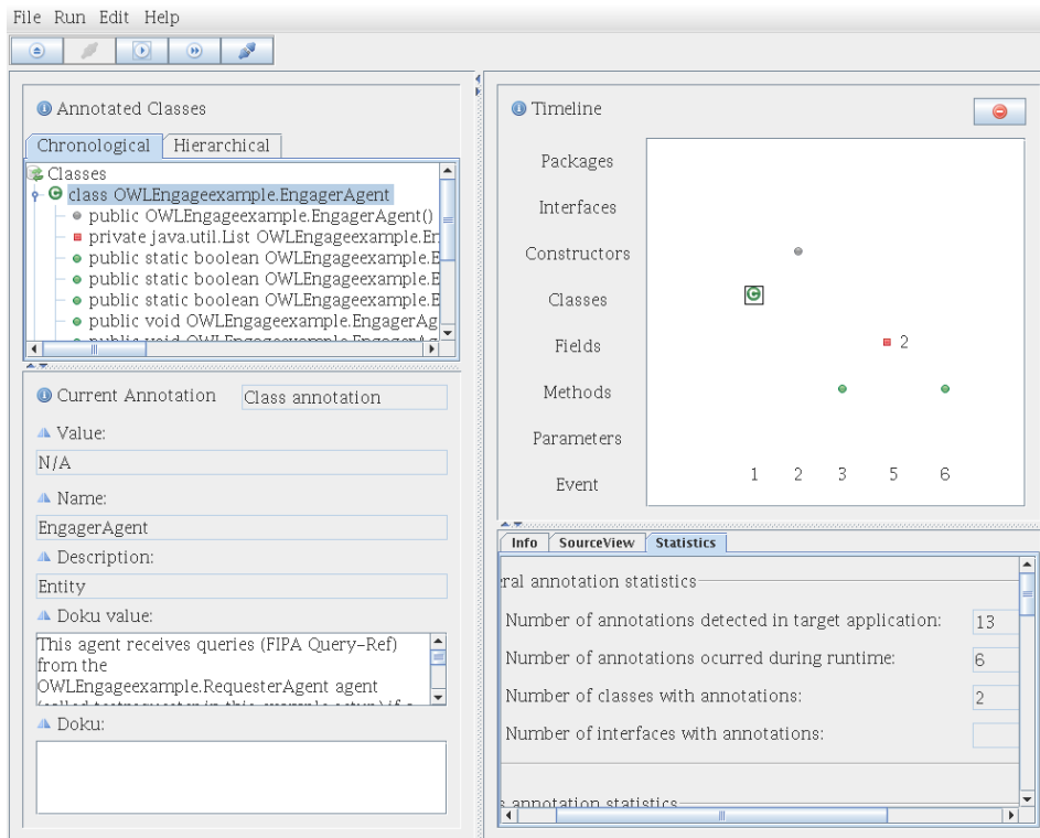
Figure 2: Screenshot of the user interface of JPAPA
