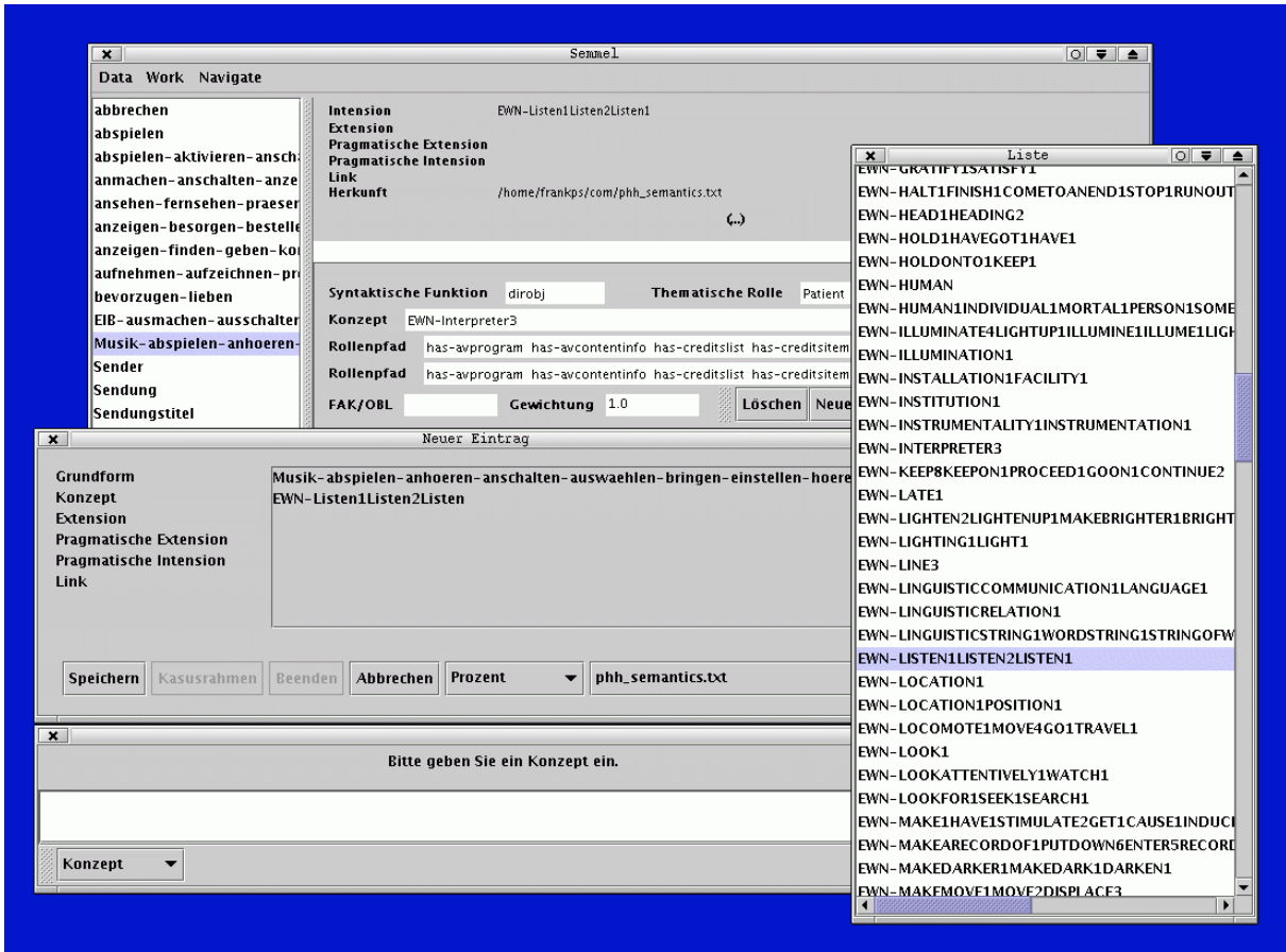
Figure 1: Lexicon-tool
